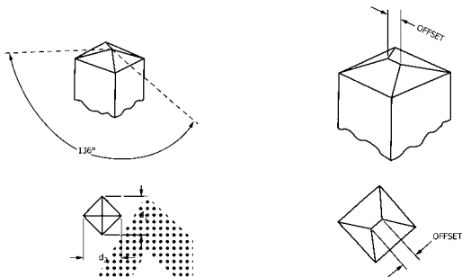
FIG. 2 Vickers Indenter
