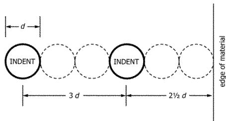
FIG. 3 Schematic of Minimum Indentation Spacing
