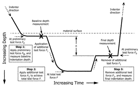
FIG. 1 Rockwell Hardness Test Method (Schematic Diagram)
